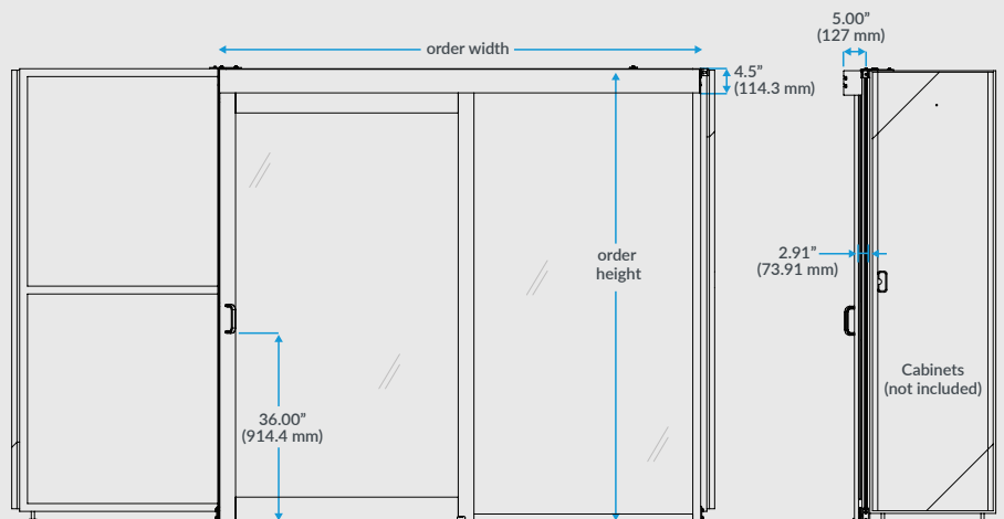
Front View NTS
