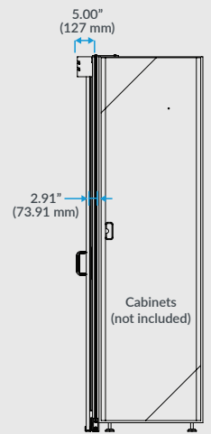
Side View NTS
