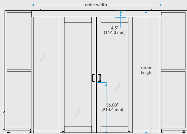
Front View NTS
