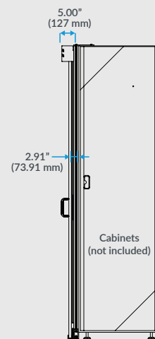
Side View NTS
