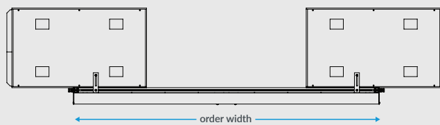
Top/Plan View NTS
